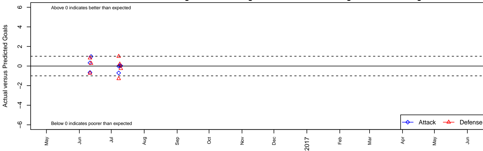
Black Angels -Unk B03 Dots are actual minus expected GF (blue circles) and GA (red triangles). Blue line is smoothed change in attack strength. Red is smoothed change in defense strength.
